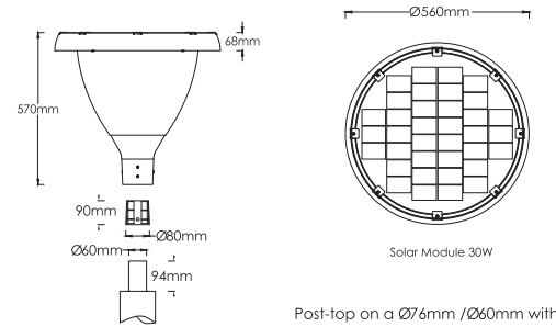
Post-top on a 76mm / 60mm with 94mm long spigot - 8 x M8 screws
